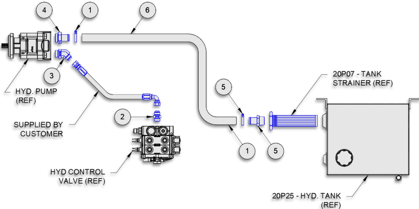
PUMP CIRCUIT
