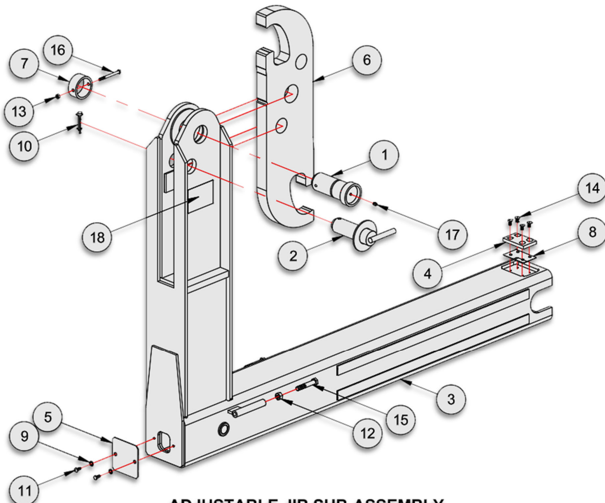
ADJUSTABLE JIB SUB-ASSEMBLY
