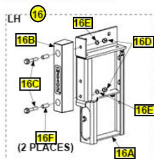
DUAL NO STEP ASSEMBLY WITH BUMPER
