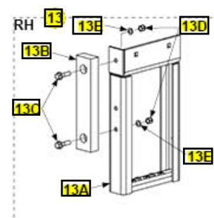
SINGLE STEP ASSEMBLY WITH PLASTIC BUMPER
