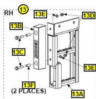
DUAL STEPS ASSEMBLY WITH RUBBER BUMPER
