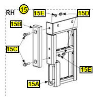
DUAL STEPS ASSEMBLY WITH PLASTIC BUMPER
